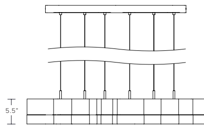
MULTI-MODULE CHANDELIER, 7 + 7
