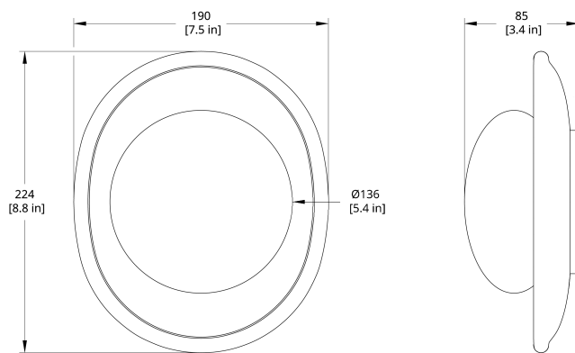
CP Crepe Large Dimensional Drawing
