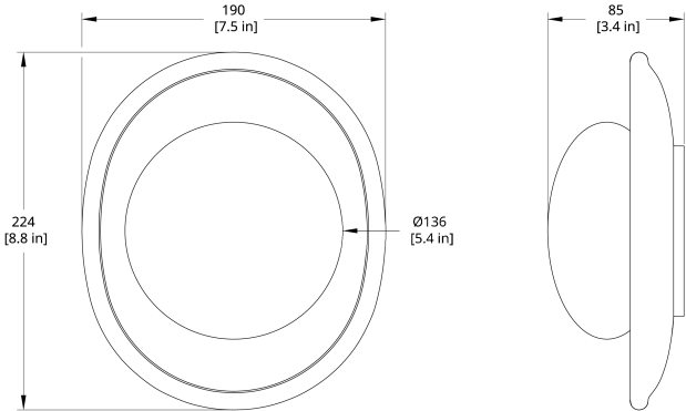
CP Crepe Small Dimensional Drawing
