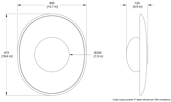
CP Crepe Large Dimensional Drawing
