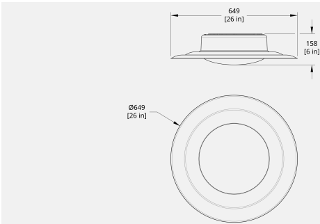
Tidal dimensional drawings
