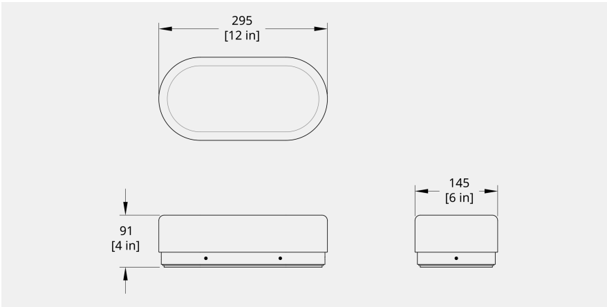
Dimple Dash dimensional drawing
