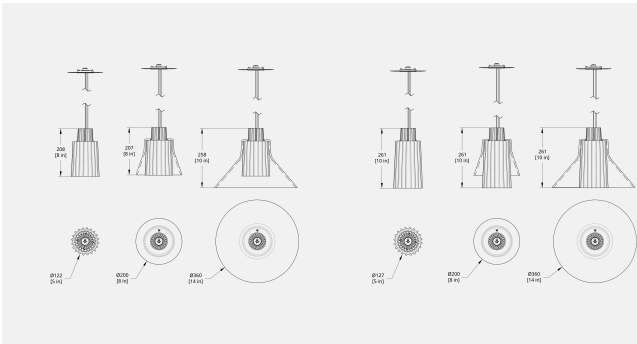
ample technical drawing, trimless canopy
